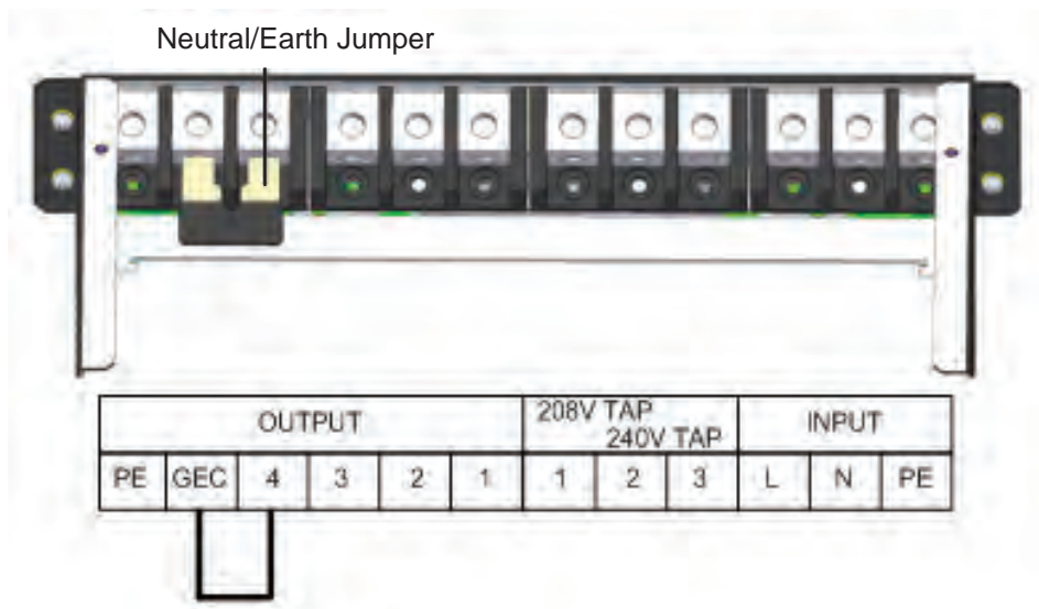
Figure 36 Configuring the neutral/earth jumper
