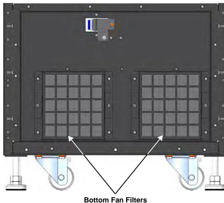
Figure 76 Replace/clean the bottom fan filter
