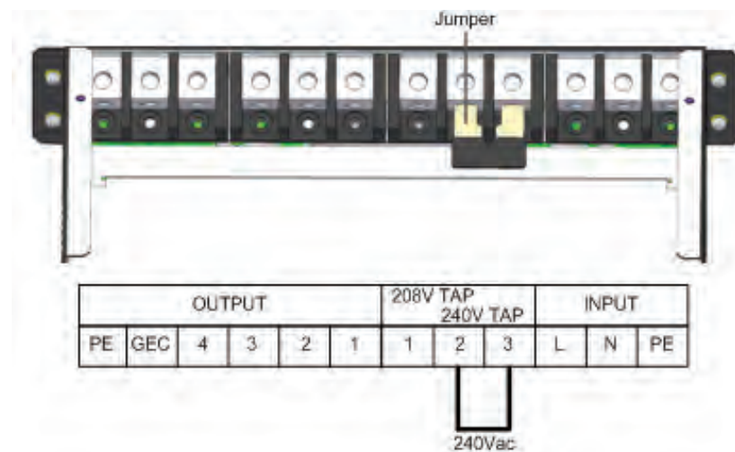
Figure 35 Setting bypass voltage jumper (200/220/230/240VAC)
