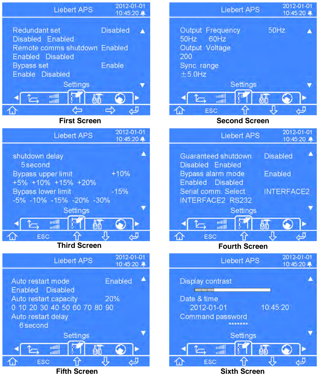
Figure 62 Settings screens
