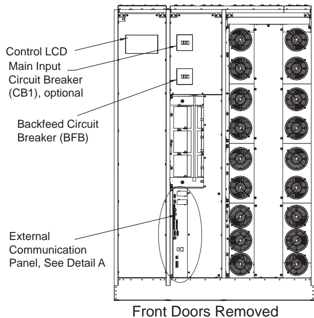
Figure 9 Main components, 225-300kVA Liebert NX UPS, SMS and 1+N multi-module unit with static bypass
