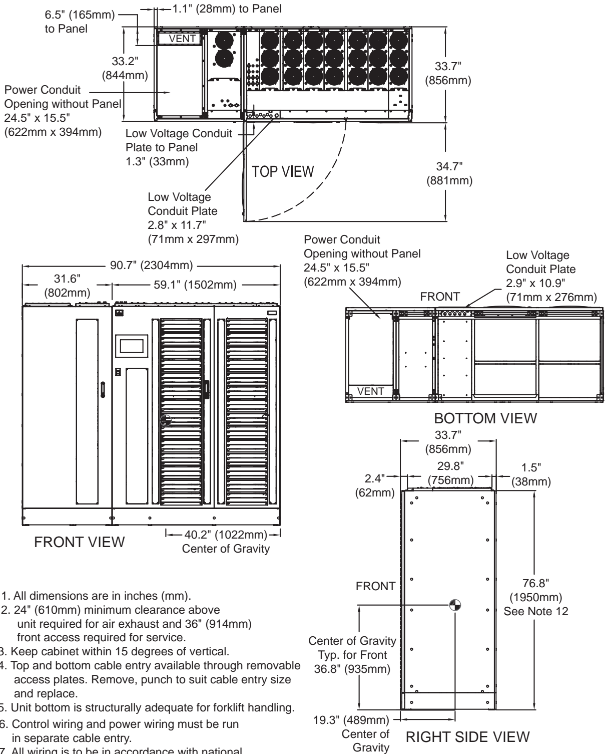
Figure 16 Outline drawing, 400-600kVA Liebert NX, SMS and 1+N multi-module unit with static bypass
