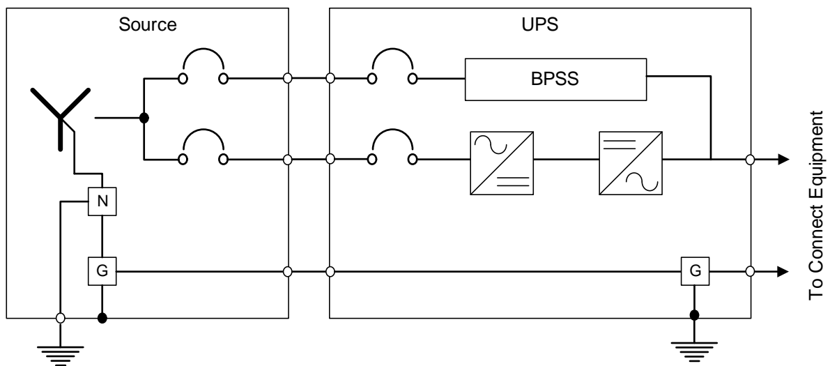
Figure 3 Grounding diagram—Three-wire single-module systems
