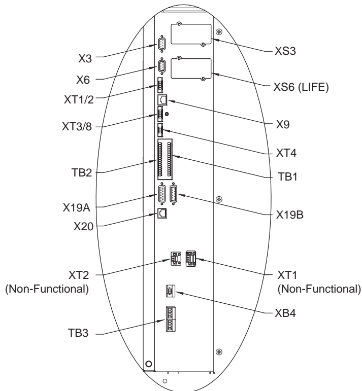
Detail A
