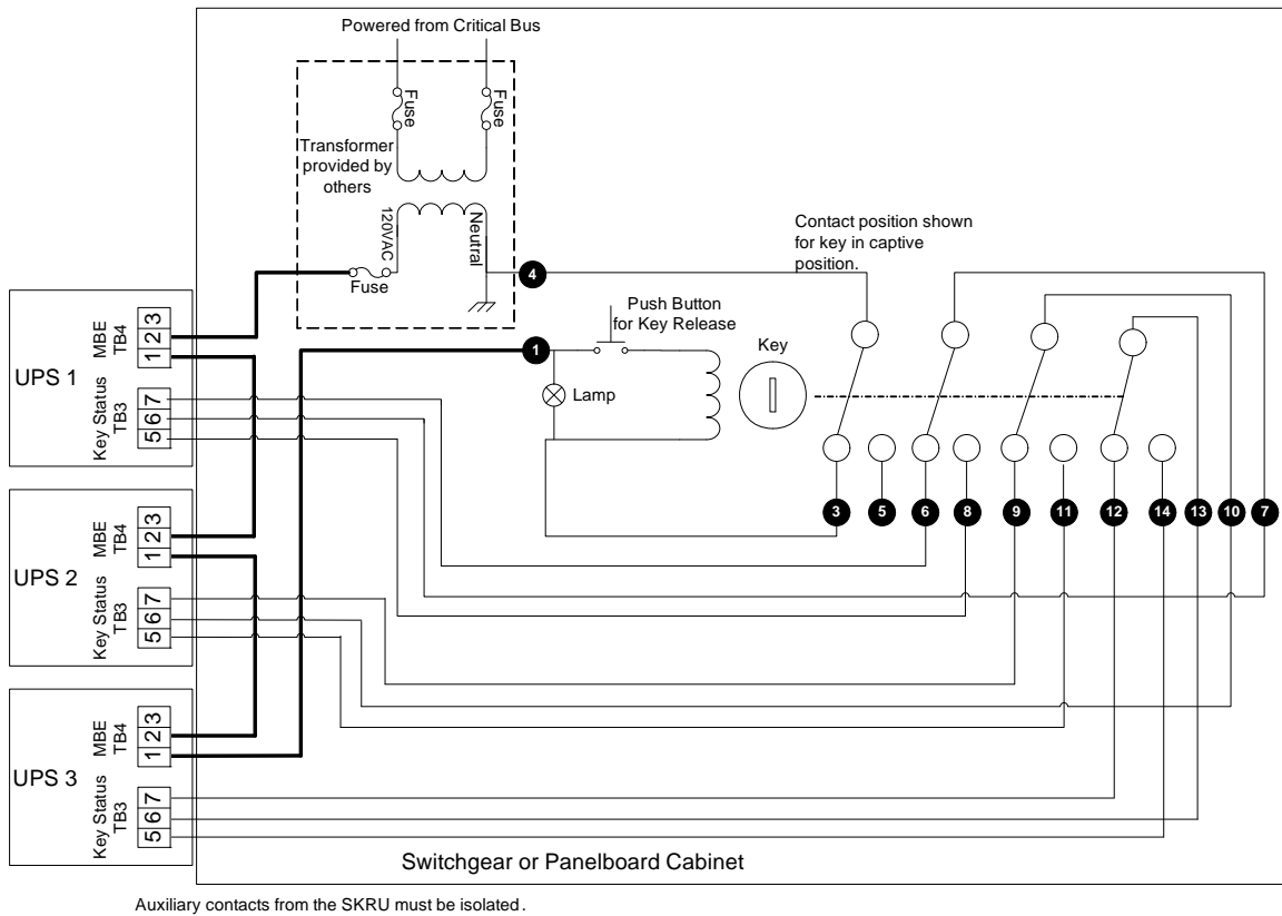
Figure 7 Control wiring
