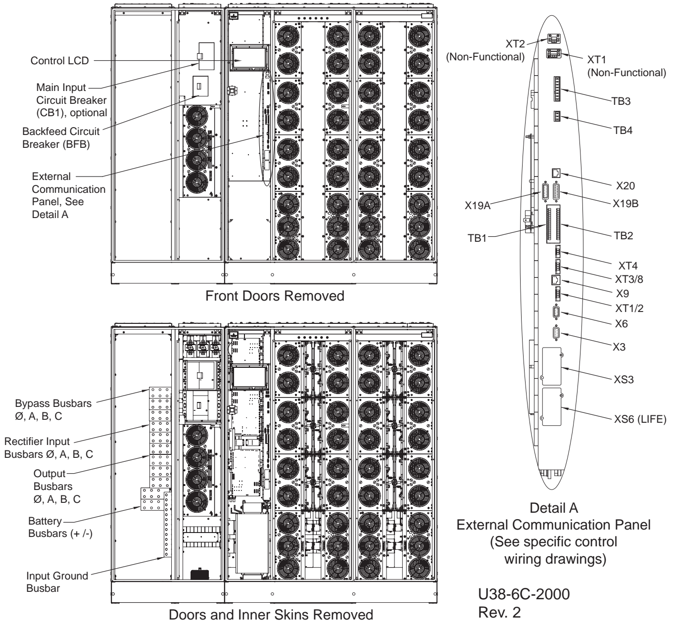
Figure 15 Main components, 400-600kVA Liebert NX UPS, SMS and 1+N multi-module unit with static bypass
