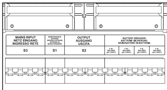
ИБП Trimod® 10/15/20
