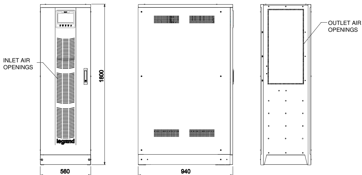
Picture 4 – Overall dimensions
