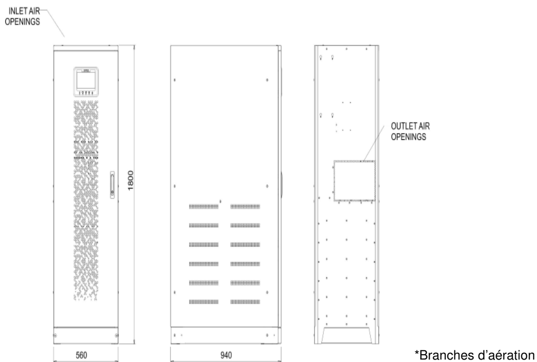
Illustration 4 – Dimensions globales
