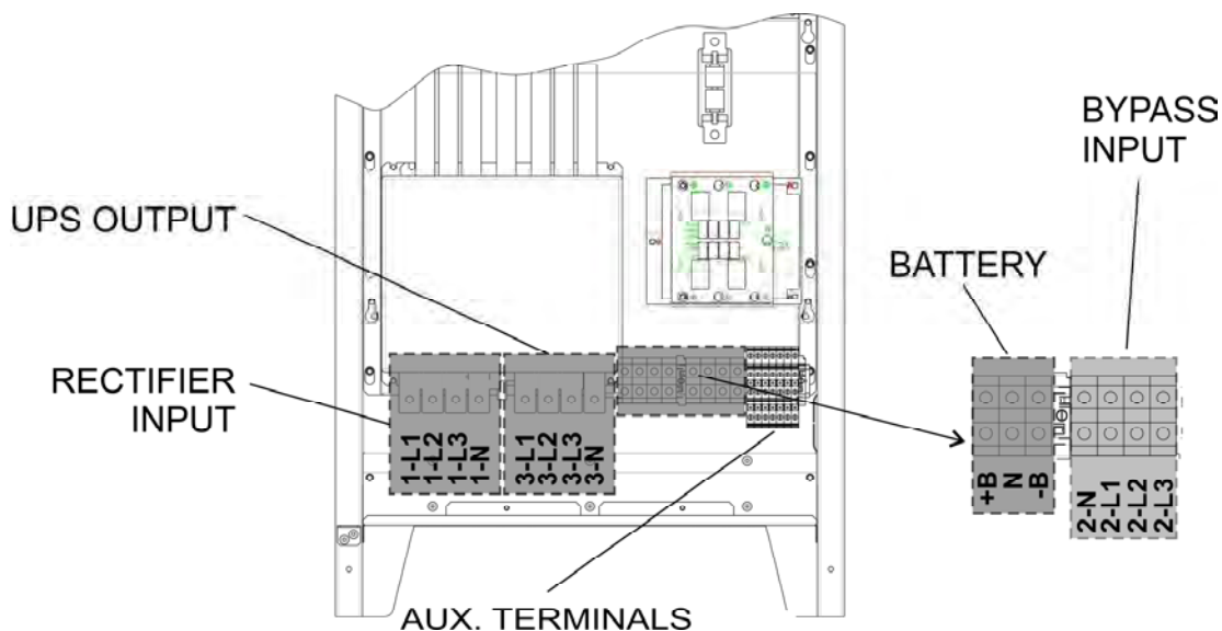
Picture 8 – Terminal board KEOR HPE 100 kVA
