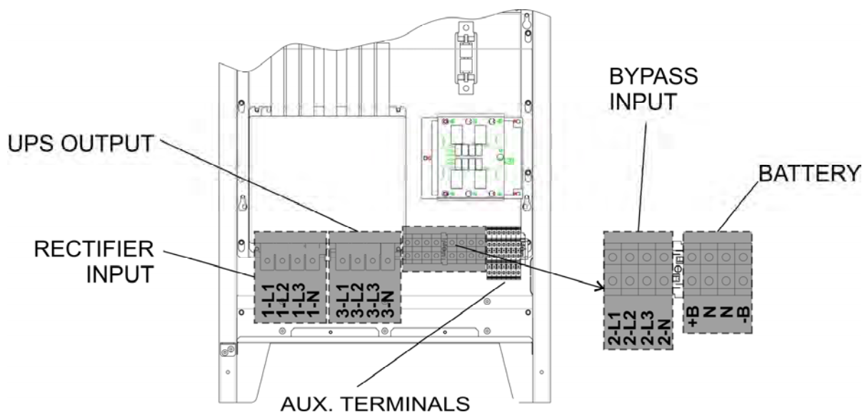
Picture 7 – Terminal board KEOR HPE 60-80 kVA
