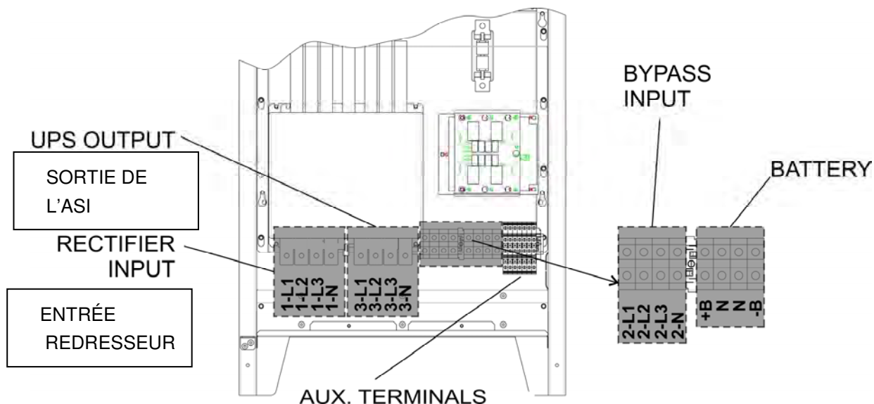
Illustration 7 – Borniers KEOR HPE 60-80 kVA
