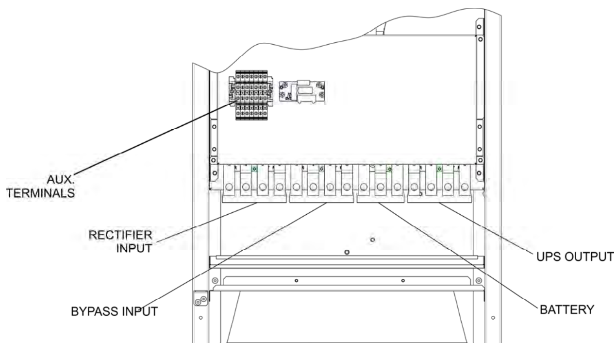
Picture 8bis – Terminal board KEOR HPE 125÷160 kVA
