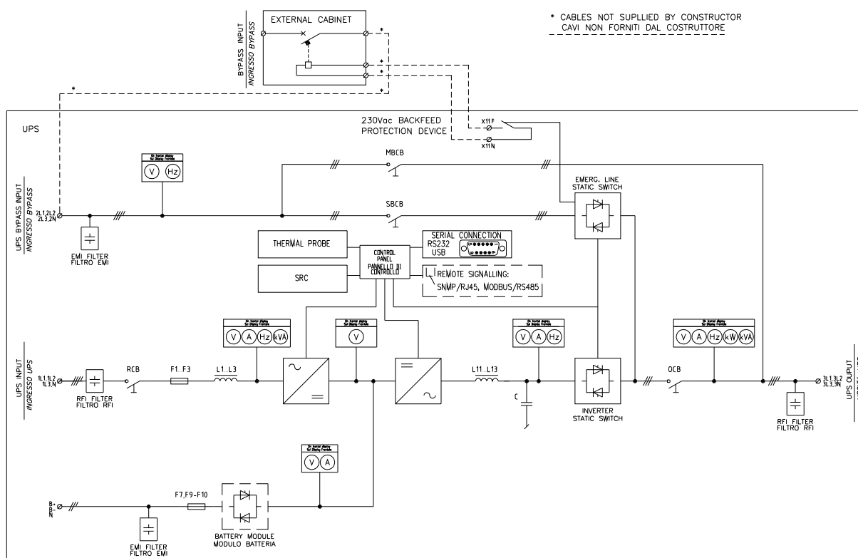
Picture 6a – Single Line Diagram KEOR HPE 100kVA with connection to external device
