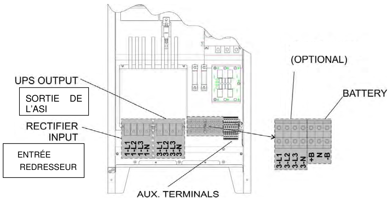
Illustration 7 – Borniers KEOR HPE 60-80 kVA
