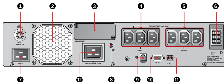
Задняя панель: UPS302R2RT0B035/ UPS302R2RT0B1B1/ UPS302R2RT0B0B6
