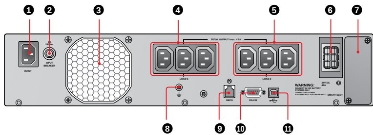
Задняя панель: UPS102R2RT0B035/ UPS102R2RT0B1B1/ UPS102R2RT0B0B6
