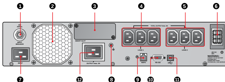
Задняя панель: UPS202R2RT0B035/ UPS202R2RT0B1B1/ UPS202R2RT0B0B6
