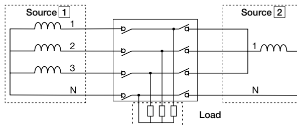
7.1.1.-6 Three phases network with neutral on source 1 Single phase network with neutral on source 2 41 NBL
