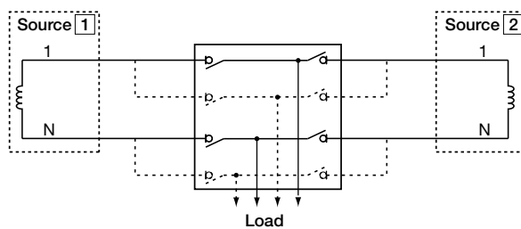
7.1.1.-4 Single phase network with neutral (phase-neutral) - 1BL*
