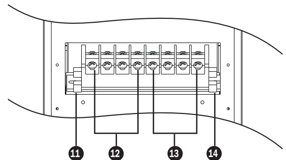
Diagram 3: SVT30KX Rear Panel
