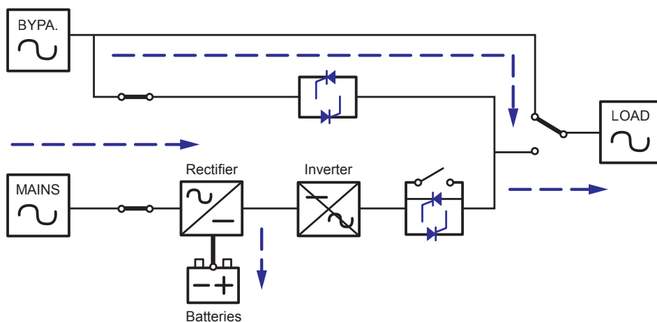
(Figure 5-6: Path of Electrical Power through the UPS in Manual Bypass Mode)
