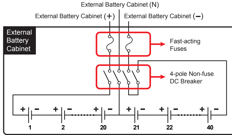
(Figure 3-19: Non-Tripp Lite External Battery Cabinet Connection)
