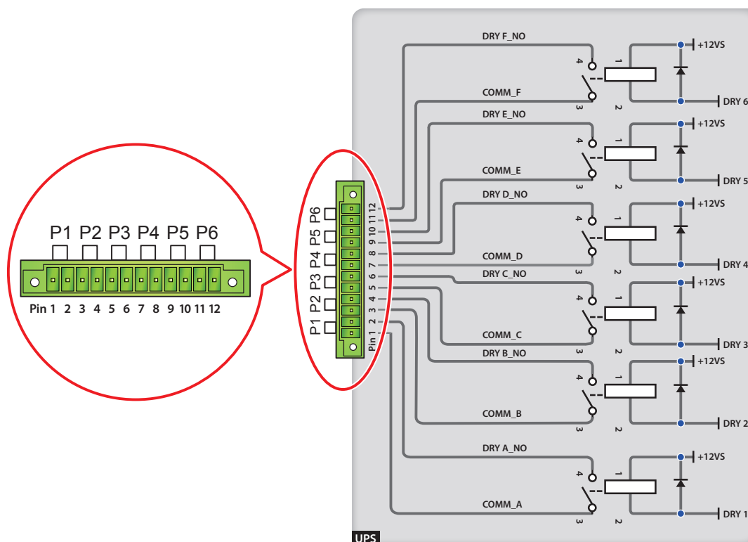
(Figure 6-4: Output Dry Contacts: Pin Definition and Design)
