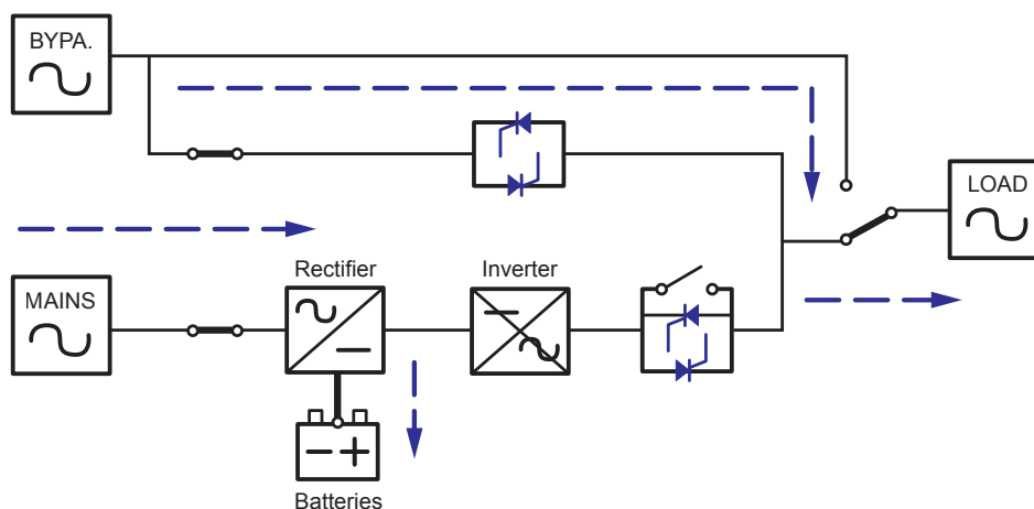
(Figure 5-5: Path of Electrical Power through the UPS in Bypass Mode)
