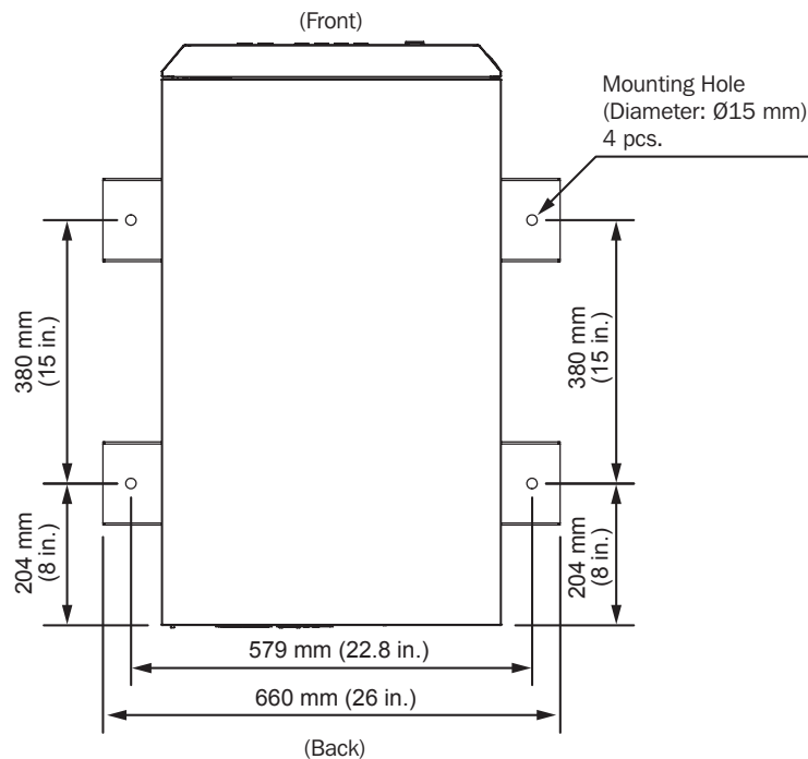
(Figure 3-2: Mounting Hole Diagram)
