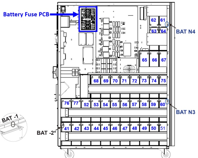
Right Side S3M30KX/S3M40KX
