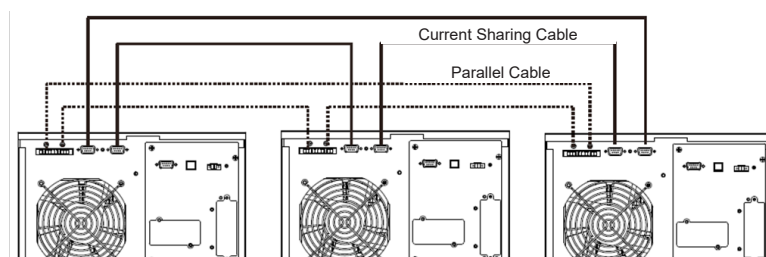
S3M30KX, S3M40KX S3M30KX/NIB and S3M40KX/NIB Parallel System UPS Wiring
