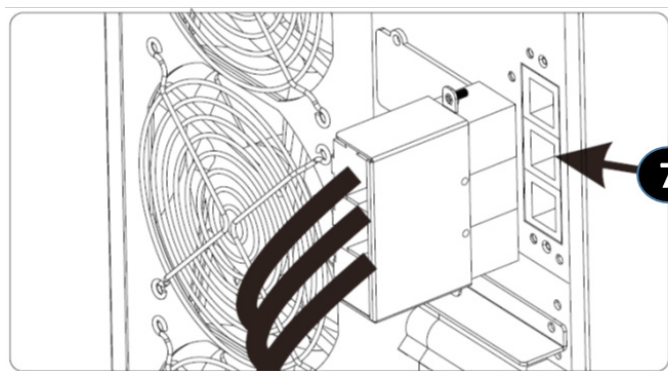
S3M30KX/NIB and S3M40KX/NIB External Battery Connection
