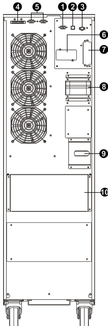
S3M40KX Rear Panel
