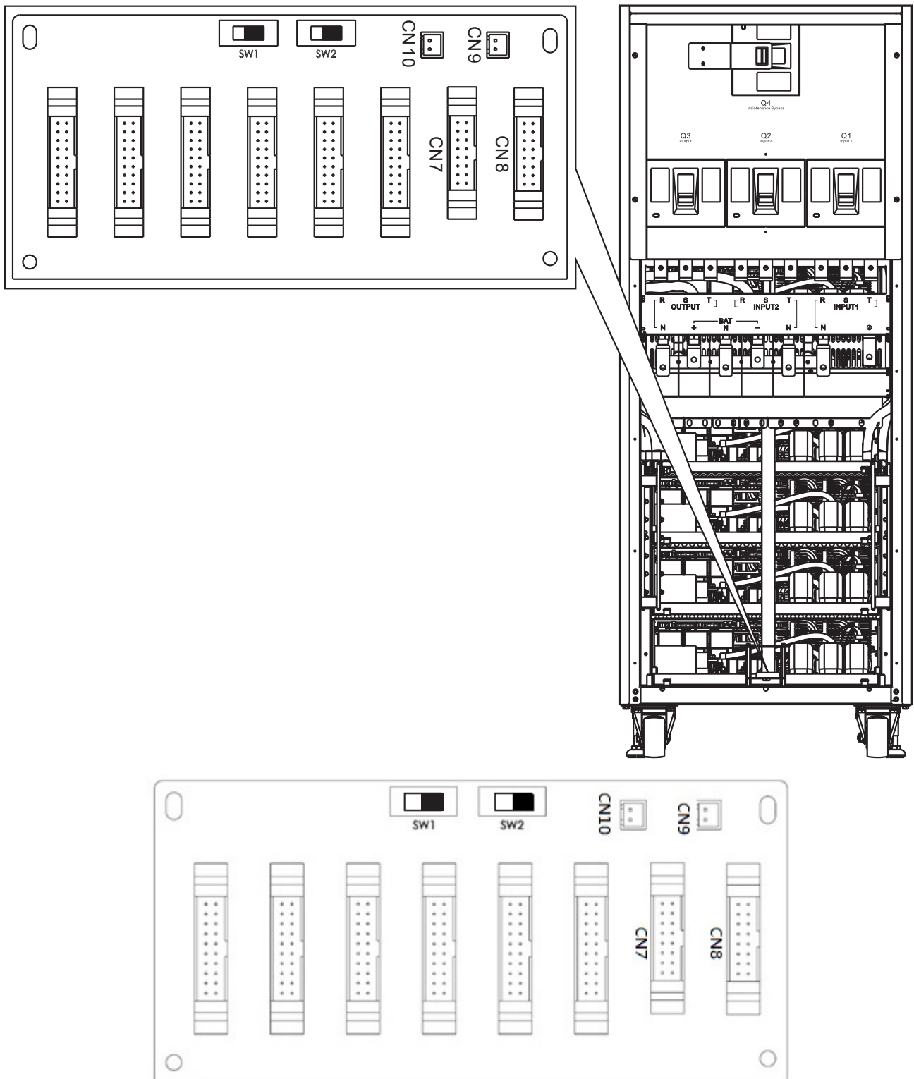
Figure 3.8 SW2 Position on UPS 1 (Default Setting)
