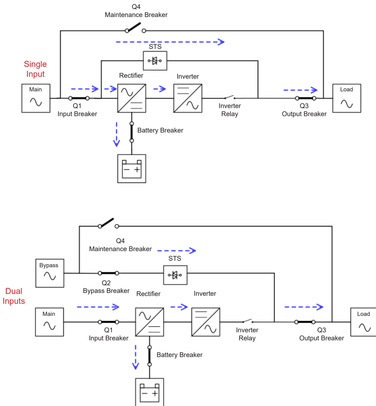
ECO Mode Diagrams
