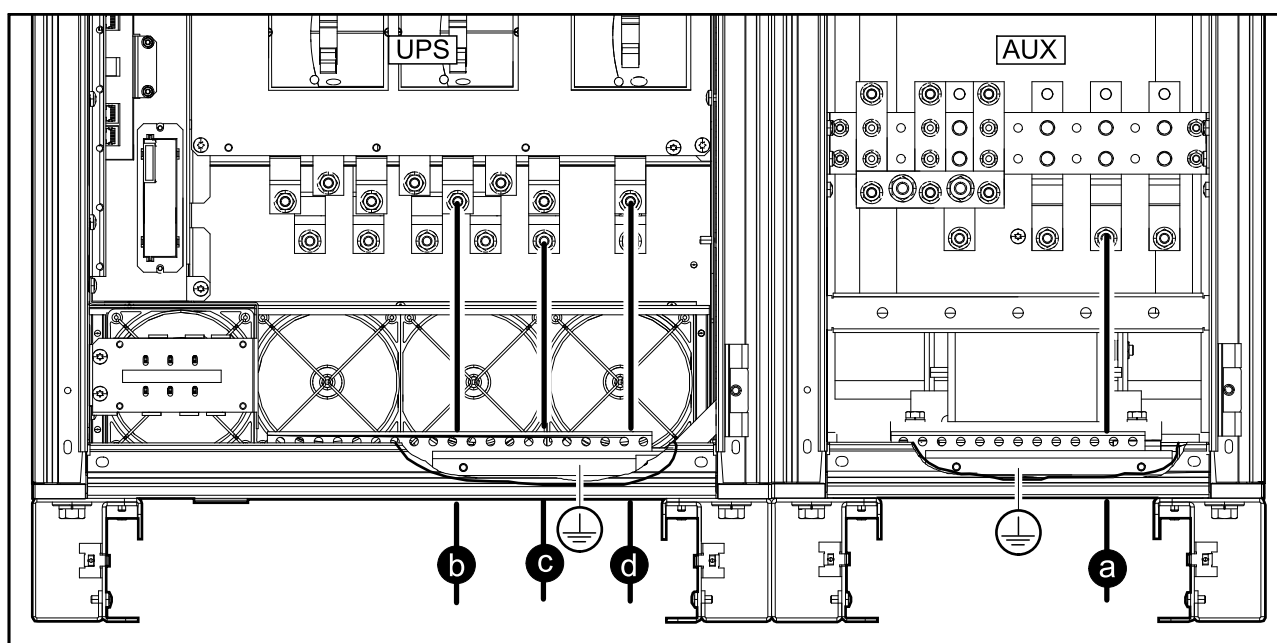
Front View of the 10–40 kVA UPS and AUX Cabinet with Bypass Transformer — 3:3
