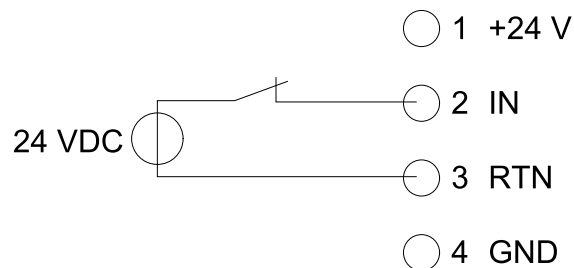
Using an External Supply
