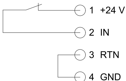
Using the Internal Supply
