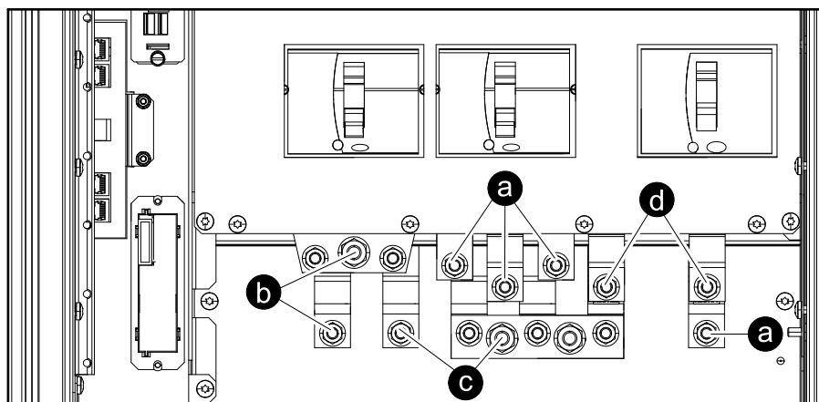
Front View of the 50–80 kVA 3:3 UPS
