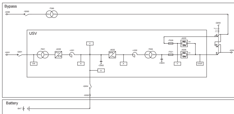
Single-phase drawing
