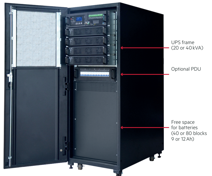
"Cabinet Plus" (UPS frame and batteries)
