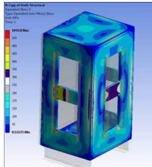
Mechanical stress simulation
